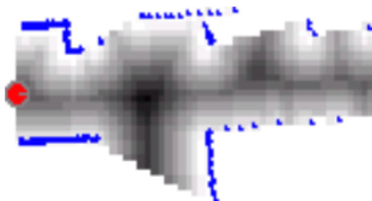
Figure 2: Likelihood Function Generated
