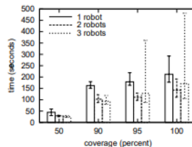
Figure 10: Results from Obstacle-Free Environment
