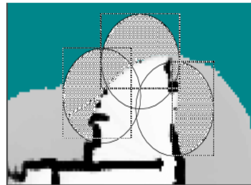
Figure 4: Expected Information Gain Information gain regions for several representative frontier cells. Circles indicate sensor range. Cross-hatched areas are information gain regions. Dotted lines are the rectangular approximations.
