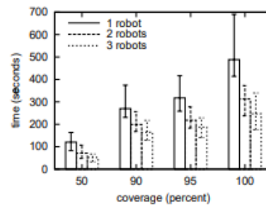
Figure 9: Results from 15% Random Obstacles
